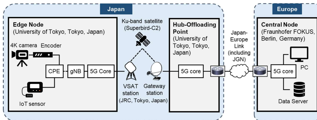
Figure 1: System configuration of the testbed in the Japan-Europe joint experiment.
