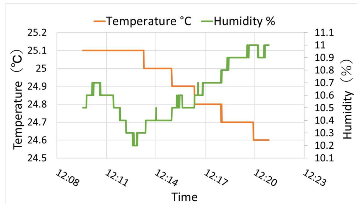
Figure 5: Transmitted IoT data results.
